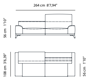
Sofá 4 plazas_ Ref. 106240
